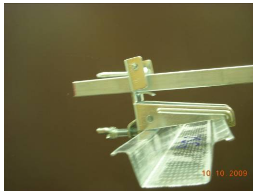
Special clip designed for trapezoid type fixed ceiling batten.
